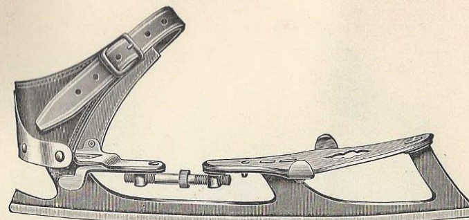
The cut above represents our Number 60 Ladies' Skate with flanged runners and side adjustment.
