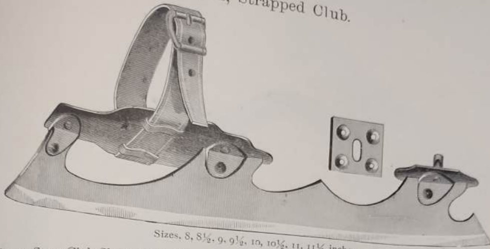
No. 2, Narrow Strap Club Skate, with Wrought Foot and Heel Plate, Riveted on to Hardened Iron Runner, Japanned. Per pair, $0.60
