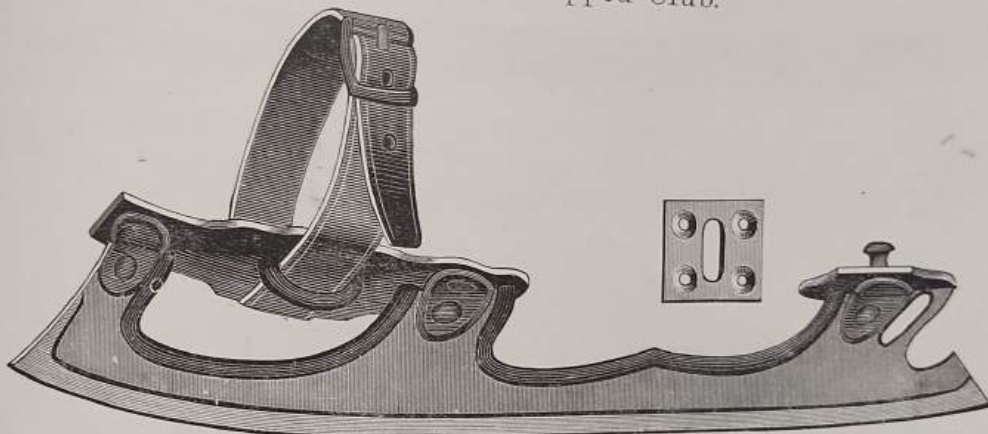
No. 2 X, Narrow Strap Club Pattern Cast Skate, Japanned, with Lower Part of Runner Finished Bright. Per pair, $0.60
