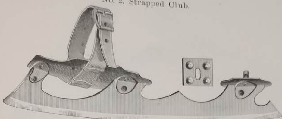
No. 2, Narrow Strap Club Skate, with Wrought Foot and Heel Plate, Riveted on to Hardened Iron Runner, Japanned. Per pair, $0.60
